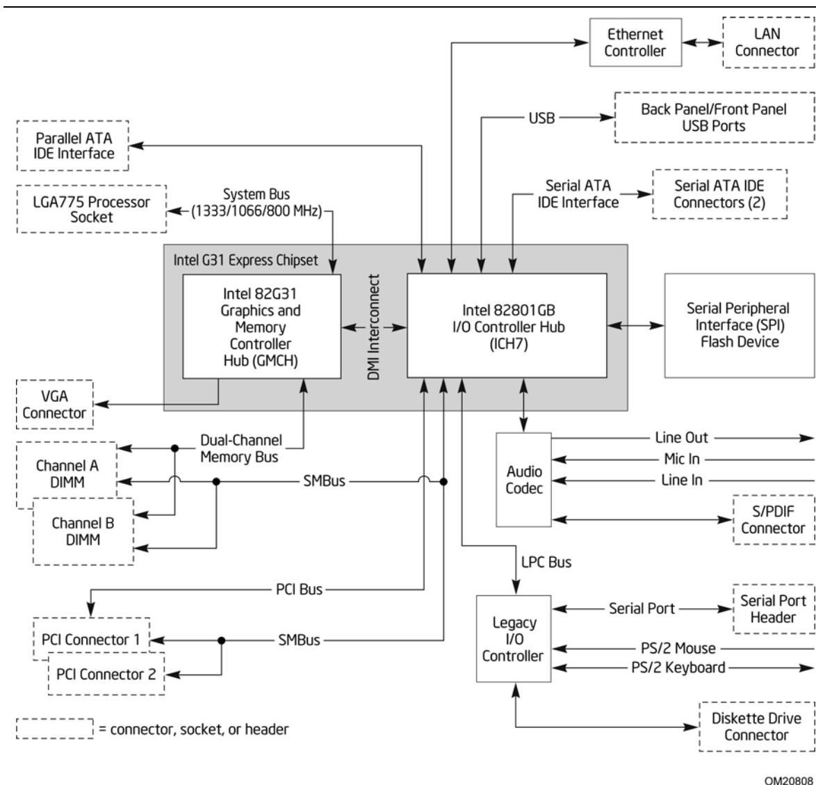
Figure 2. Block Diagram
