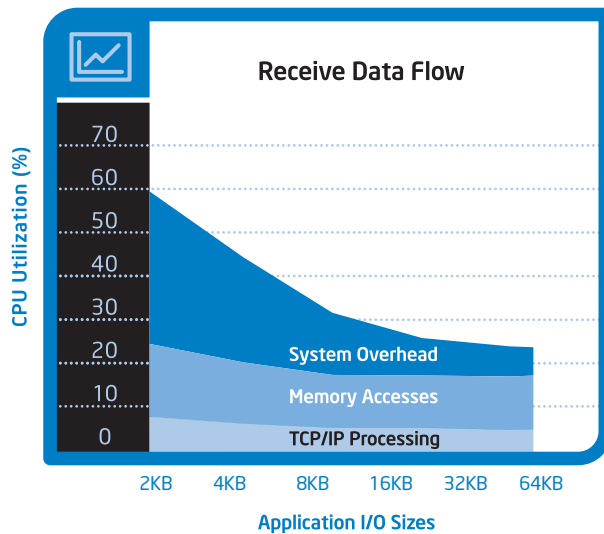
Figure 3. CPU utilization varies according to I/O size. TCP/IP processing is fairly constant and tends to be a smaller part of CPU utilization compared to system overhead.
