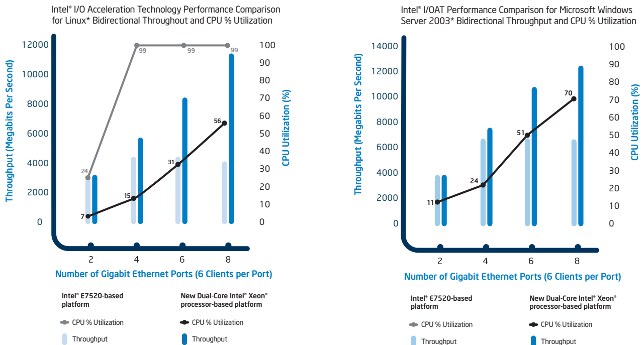
Figure 5. Network-performance comparisons for platforms with and without Intel® I/OAT. Compared to previous processors, the new Dual-Core Intel® Xeon® processor with Intel® I/OAT provides superior performance in terms of both higher throughput and reduced percentage of CPU utilization.
