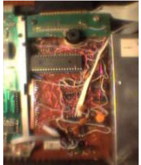
THE FLOPPY DISK CONTROLLER BOARD. IT SITS BETWEEN THE MAIN CPC BOARD AND THE 3.5 INCH DISK DRIVE.
