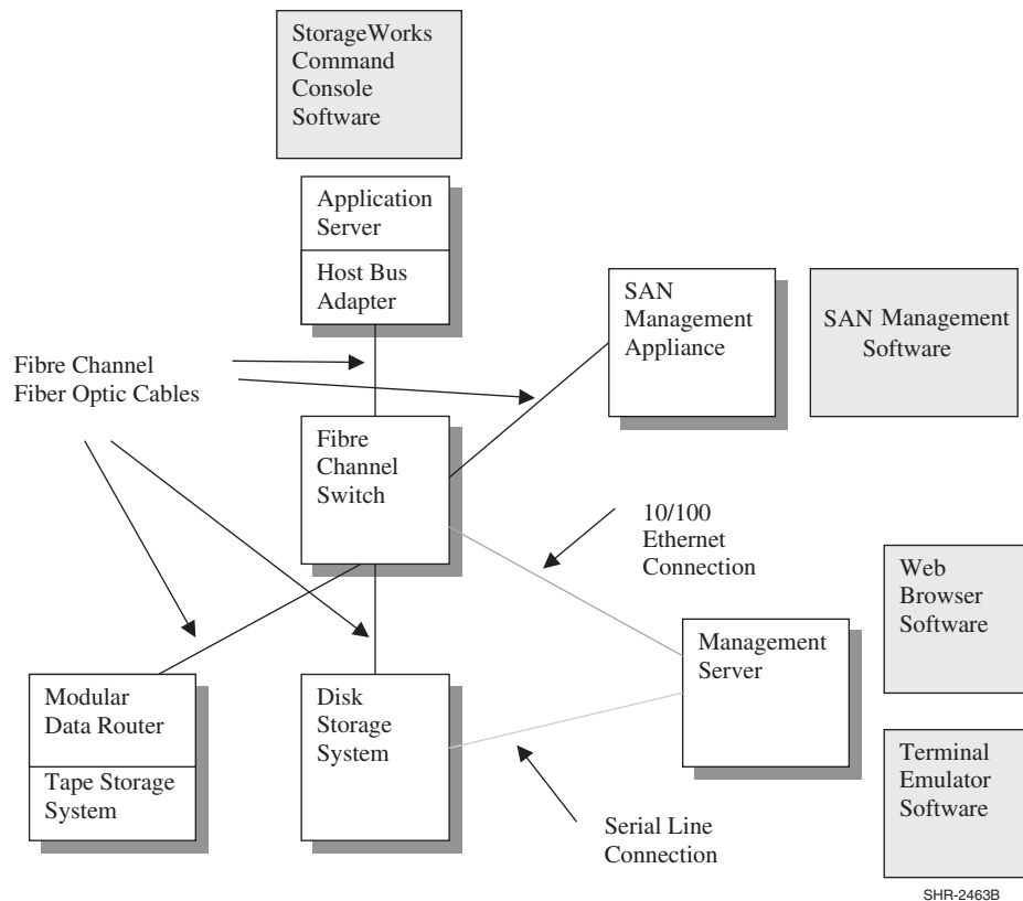
Figure 57: SAN Components
