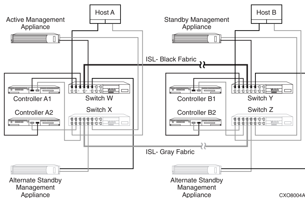
Figure 45: Continuous Access EVA basic configuration
