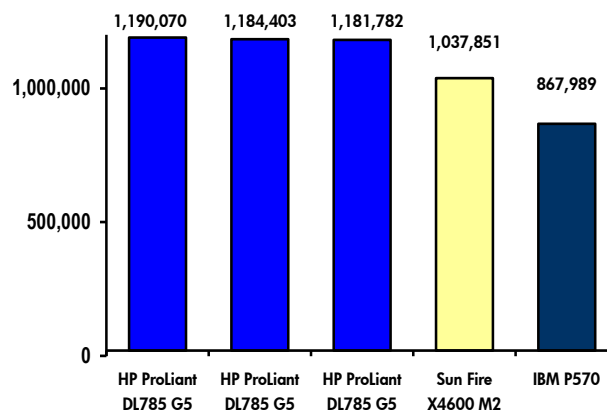
Figure 1. Top five 8-processor results on SPECjbb2005 benchmark
