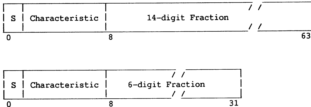
Figure 3-5. Long and Short Floating-Point Numbers
