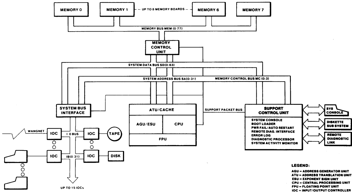
Figure 1-4. VS300 Architecture
