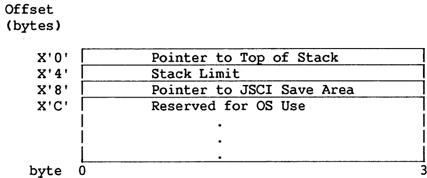
Figure 3-12. Format of Stack Header Block (SHB)
