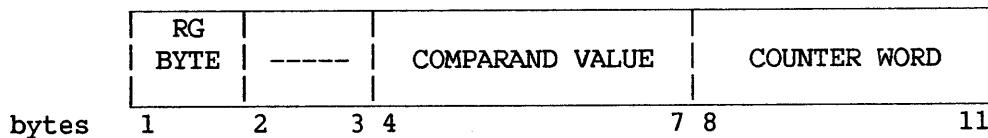
Figure 7-8. Entry for General Register Modification Trap
