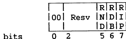
Figure 9-5. Status Qualifier Byte (SQB)
