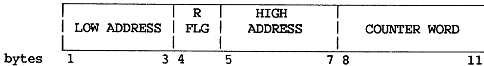
Figure 7-7. Entry for PCW Range trap
