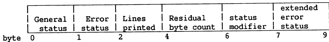
Figure 11-5. Printer IOSW Format
