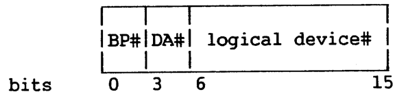
Figure 9-7. VS15, VS65 PDA
