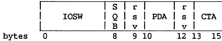
Figure 9-3. IOC Status Table (IOCST) Entry
