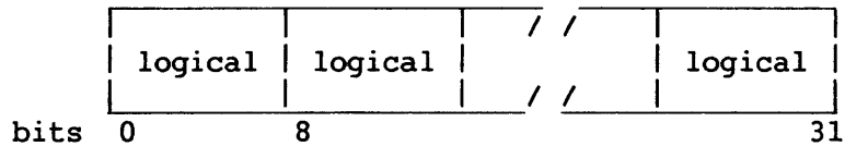
Figure 3-7. Fixed-Length Logical Operand (one to four bytes)
