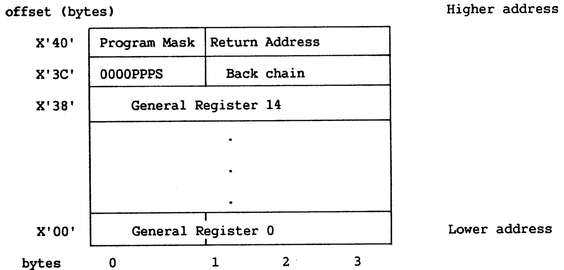
Figure 4-11. JSCI Save Area
