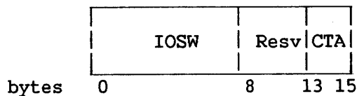
Figure 9-2. IOP Status Table (IOPST) for the VS100
