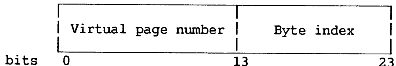
Figure 4-3. Virtual Address Format
