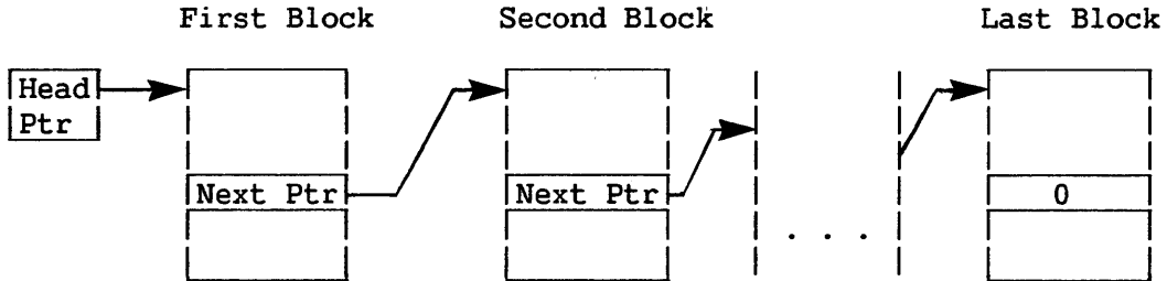
Figure 3-9. LIFO List
