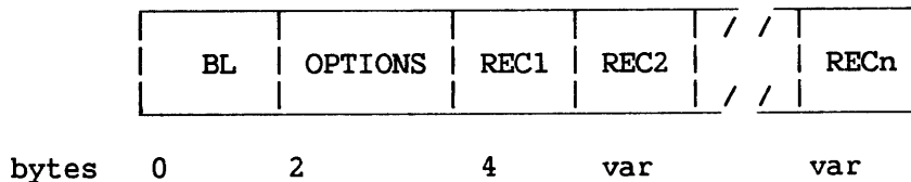
Figure 11-7. Format of the Control Data Block
