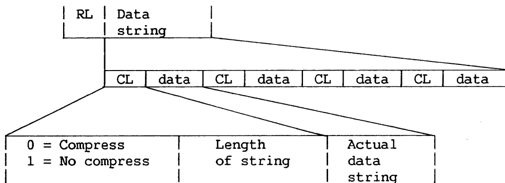
Figure 11-3. Elements of Compressed Record
