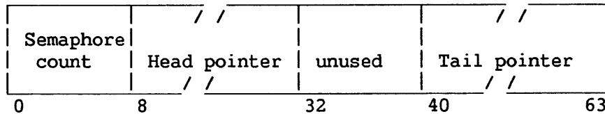
Figure 3-11. Semaphore
