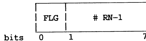
Figure 4-6. Byte 4 of SCR
