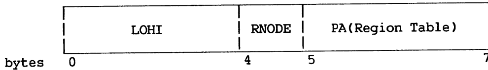
Figure 4-5. Format of SCR
