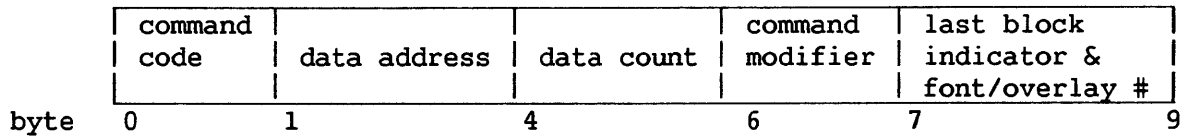
Figure 11-4. Printer IOCW
