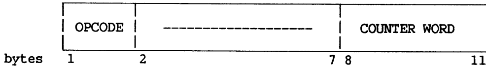
Figure 7-6. Entry for Opcode Trap
