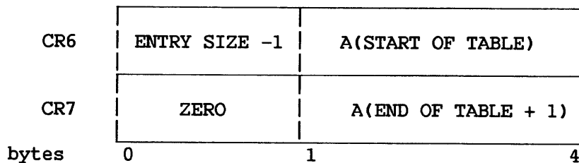
Figure 4-13. Control Registers 6-7
