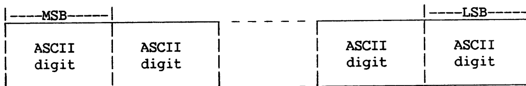
Figure 3-4. External Decimal Number Format
