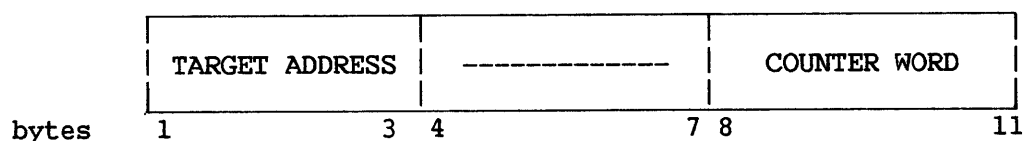
Figure 7-4. Entry for PCW Trap
