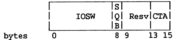
Figure 9-1. DA Status Table (DAST) Entry
