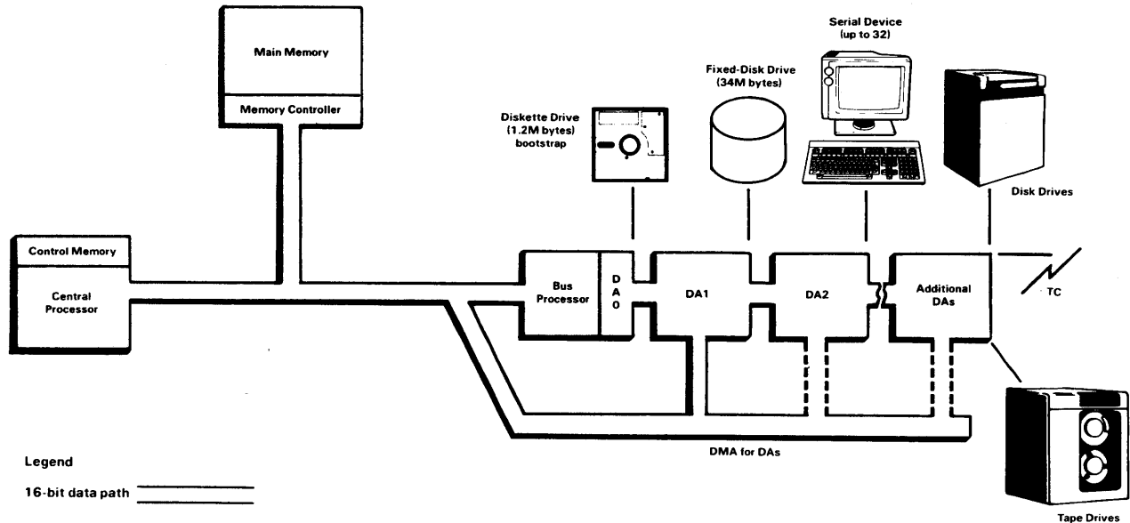
Figure 1-1. VS15 Architecture
