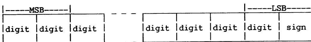
Figure 3-2. Packed Decimal Number Format
