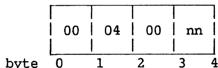
Figure 11-10. Four-Byte Font Selection Record
