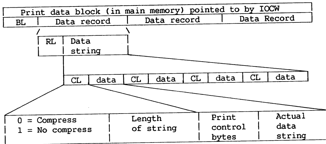
Figure 11-6. Format of Print Data Block and Record
