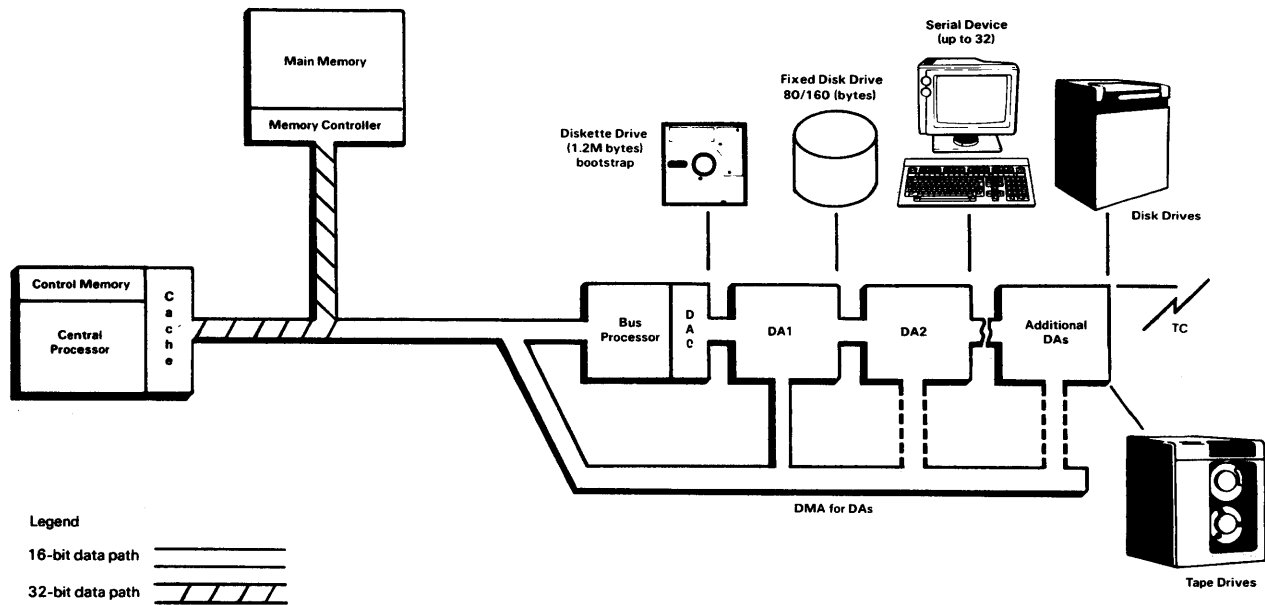
Figure 1-2. VS65 Architecture
