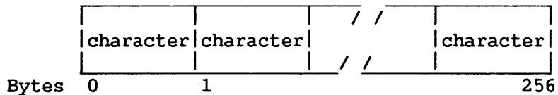
Figure 3-8. Variable-Length Logical Operand (up to 256 bytes)
