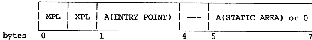
Figure 4-12. Format of Linkage Table Entry
