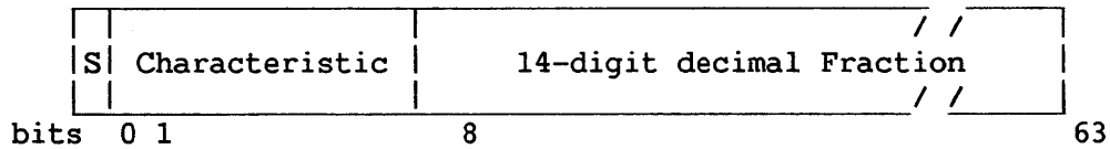
Figure 3-6. Decimal Floating-Point Number Format
