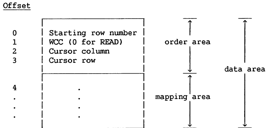
Figure 10-2. Data Area Specified by Workstation IOCW
