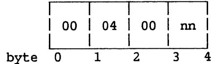
Figure 11-8. Format of Vertical Pitch Record
