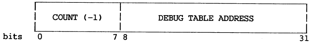
Figure 7-1. Format of Control Register 3
