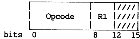
Figure 9-12. SIO, CIO, and HIO Instruction Format
