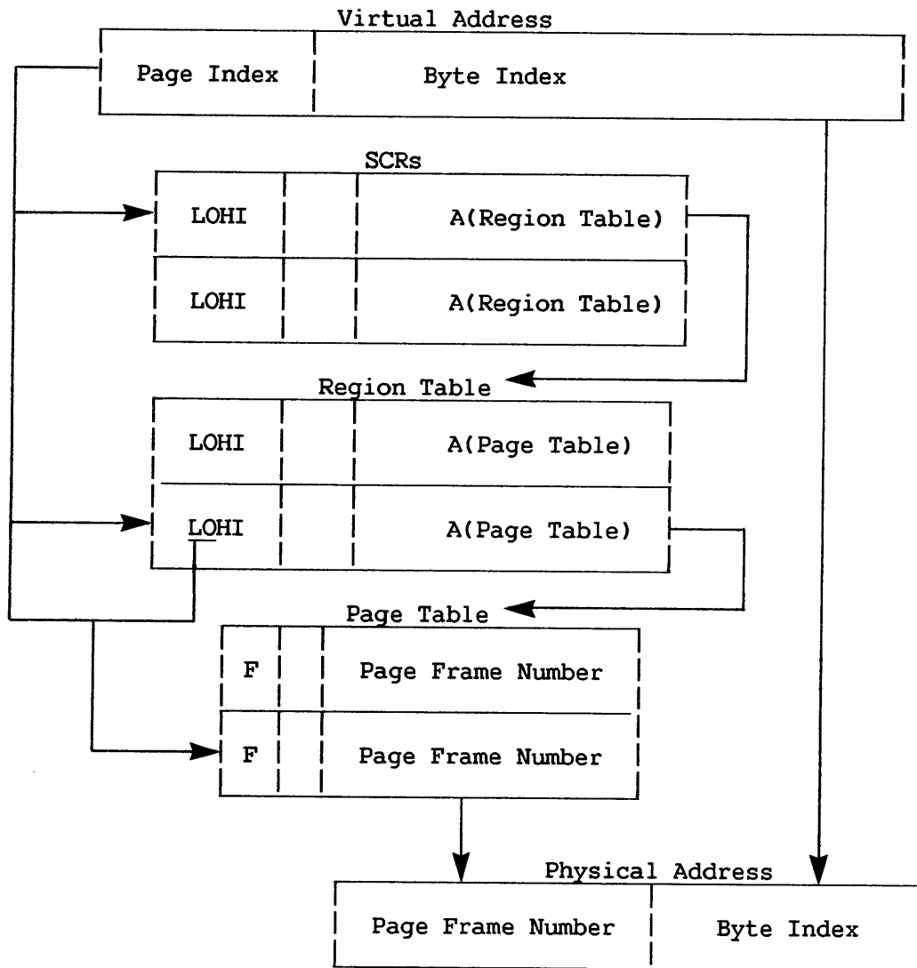
Figure 4-9. Virtual-to-Physical Address Translation
