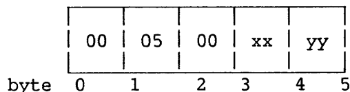
Figure 11-11. Five-Byte Font Selection Record
