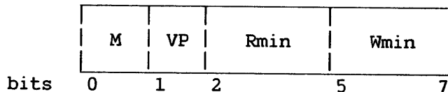
Figure 4-8. Format of MOD Byte
