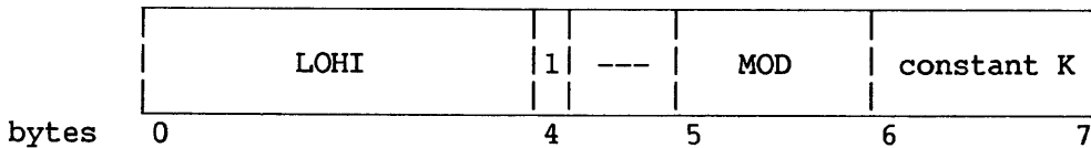
Figure 4-10. Alternate Format of SCR
