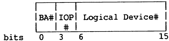
Figure 9-8. VS100 PDA
