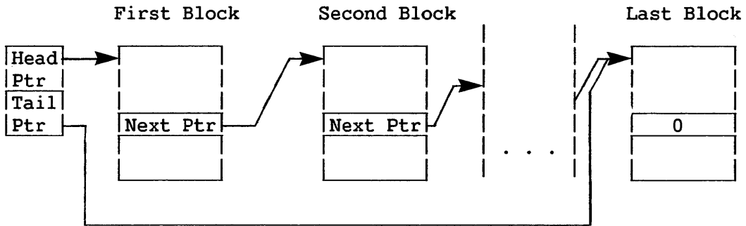
Figure 3-10. FIFO List
