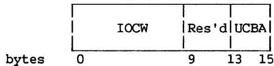
Figure 9-4. I/O Command Table (IOCT)
