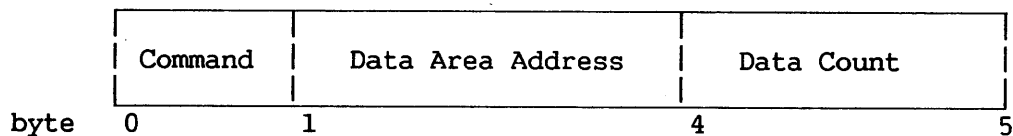
Figure 10-3. Workstation IOCW
