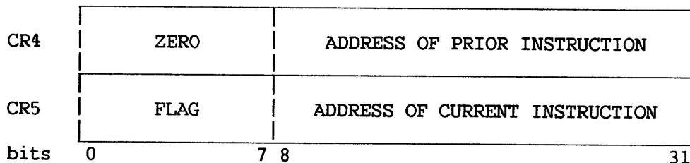
Figure 7-2. Format of Control Registers 4 and 5.
