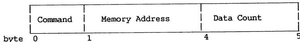
Figure 13-4. Tape IOCW
