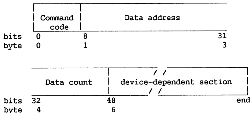
Figure 9-10. I/O Command Word (IOCW) Format
