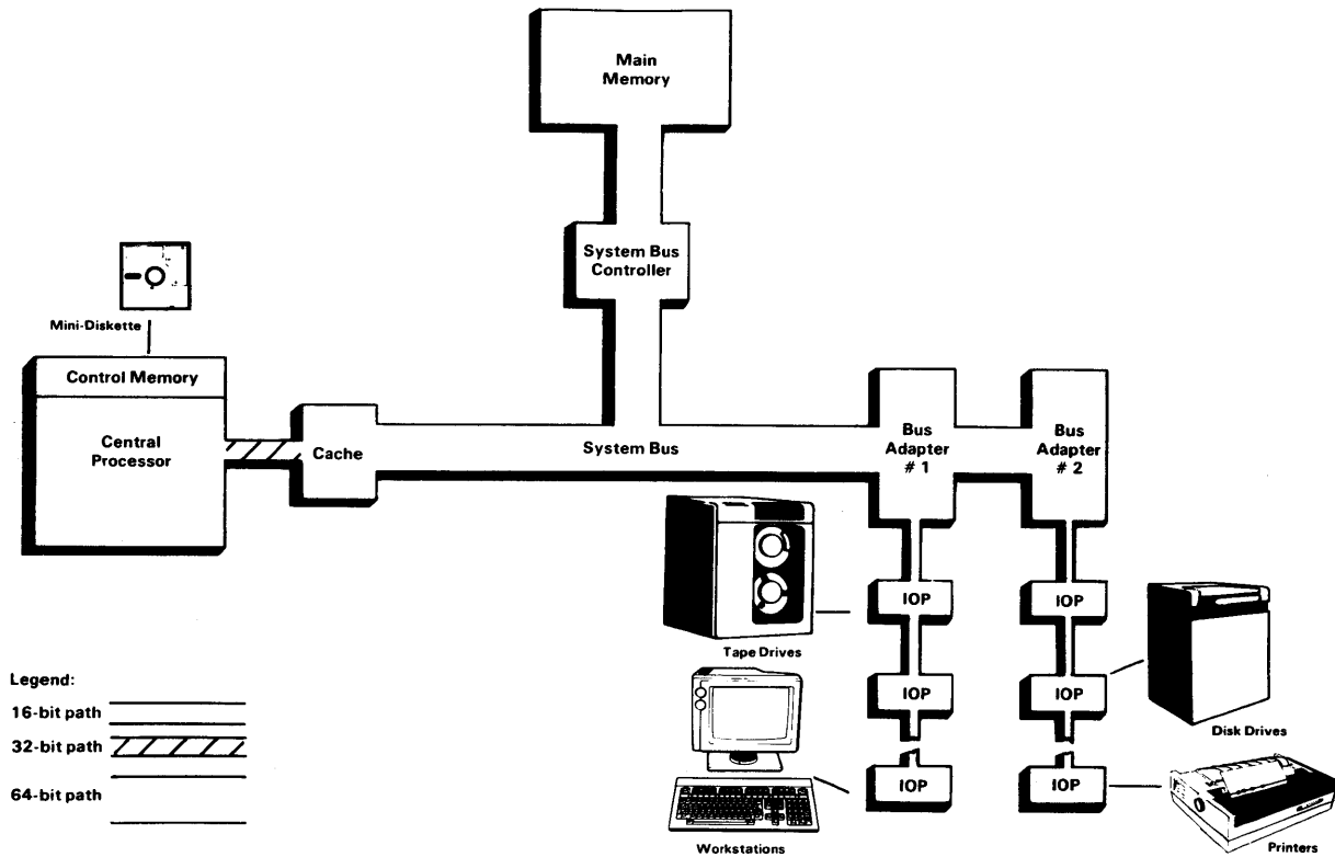
Figure 1-3. VS100 Architecture
