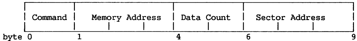
Figure 12-1. Disk IOCW
