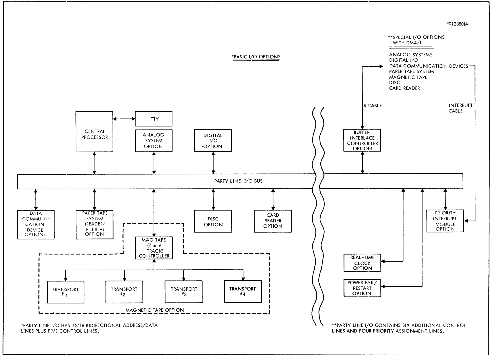
Figure 2-1. DATA 620/i Input/Output System
