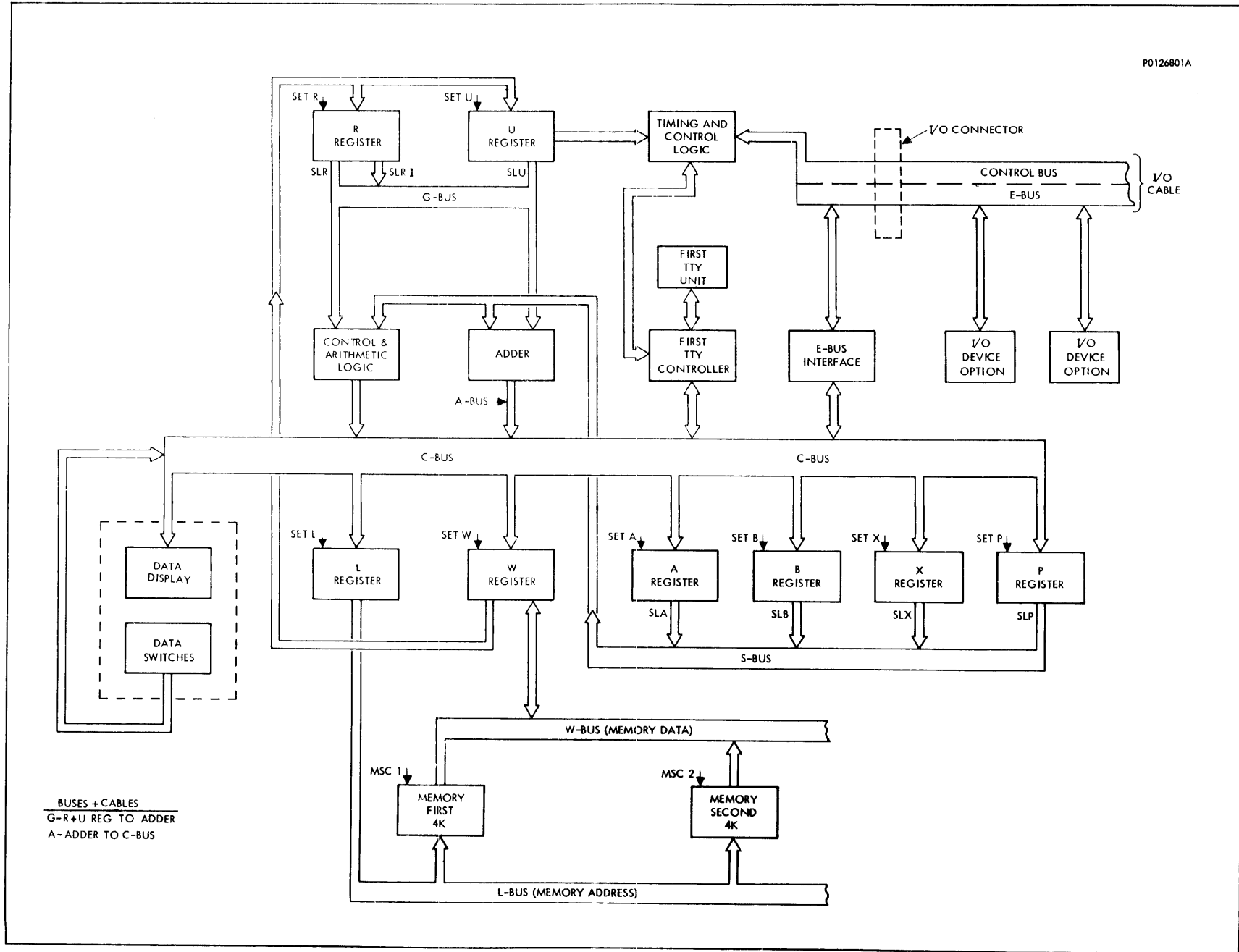
Figure 1-1. 620/i Organization
