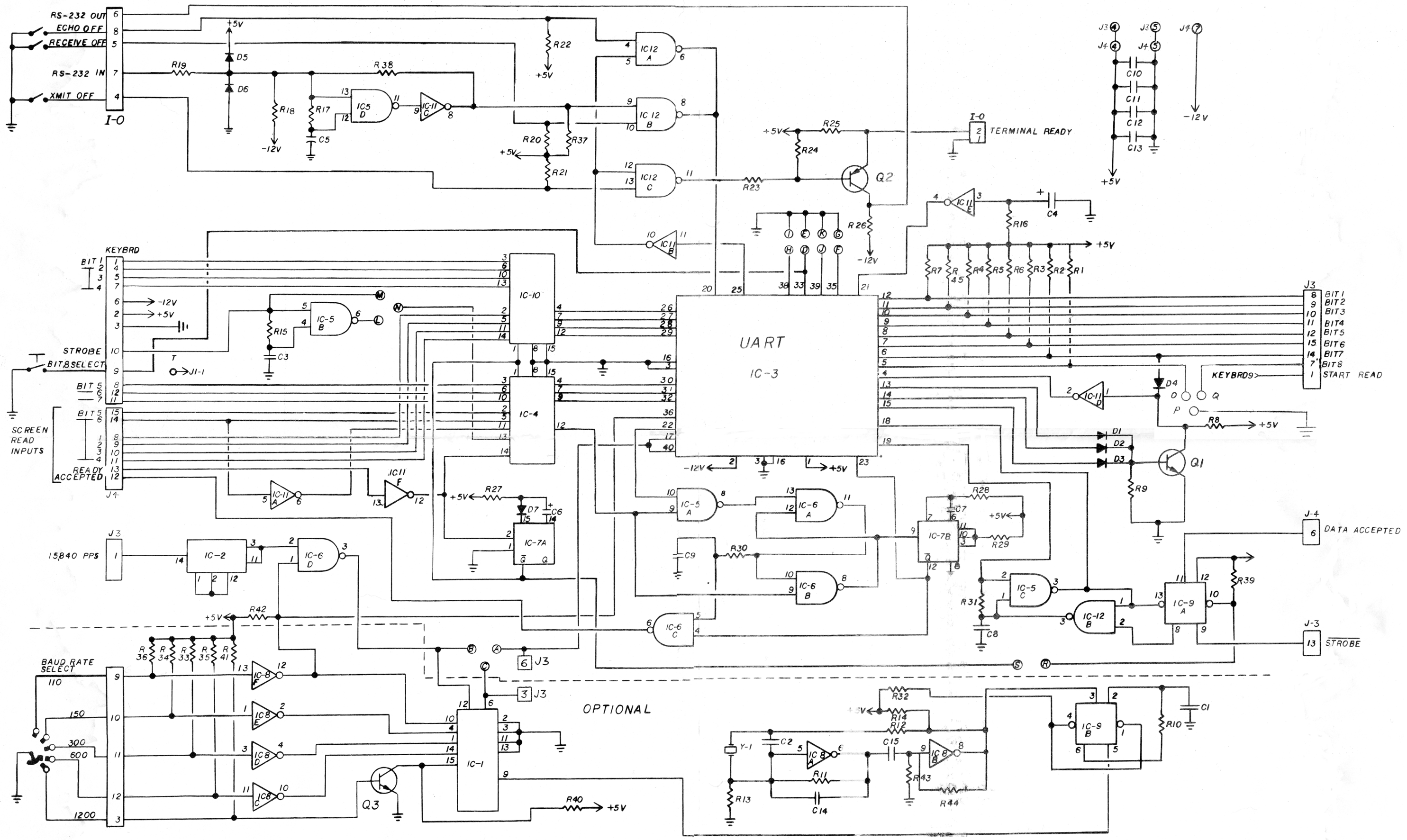
Schematic - CT-S Version 2 Serial Interface Board
