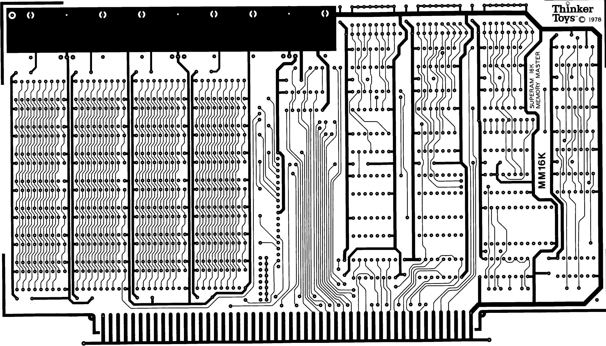
THINKER TOYS SUPERAM 16K MEMORY MASTER COMPONENT SIDE P.C. DESIGN BY M&M DESIGNS 12-78
