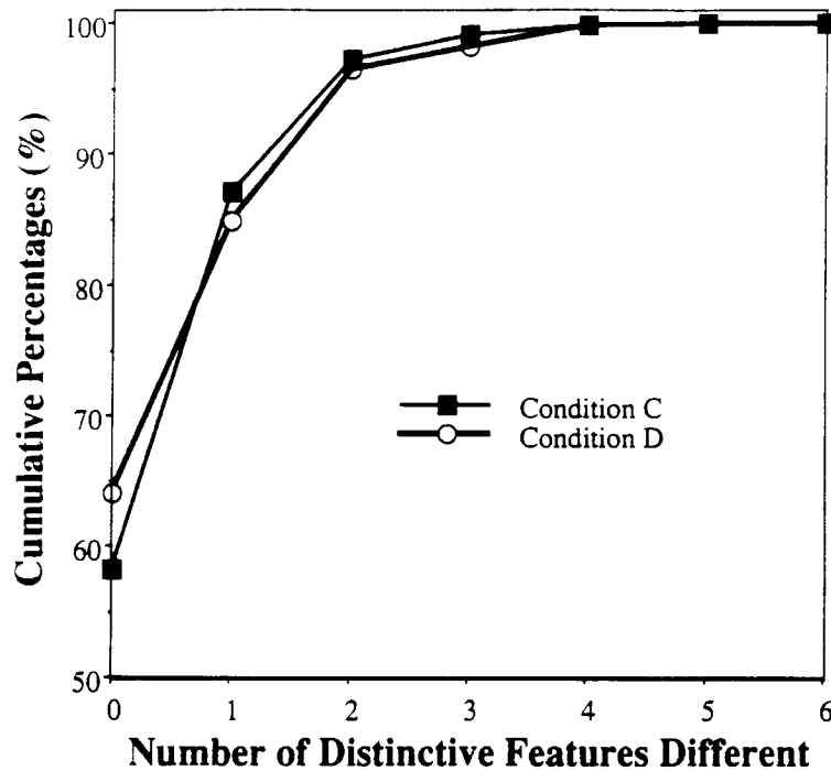
Figure 3.7: Performance of conditions C and D in terms of the number of features different between network outputs and transcription labels
