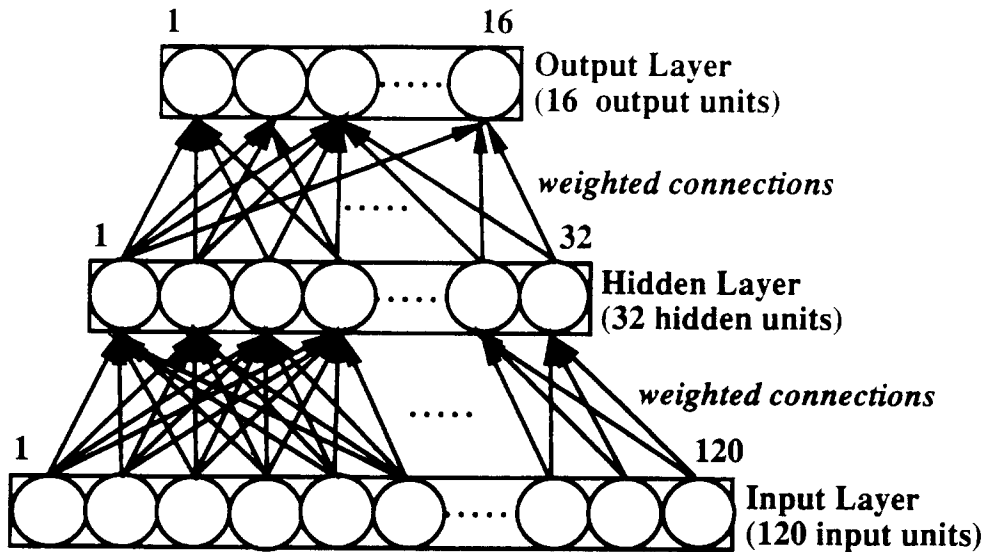
Figure 2.6: Structure of the Multi-Layer Perceptron Classifier
