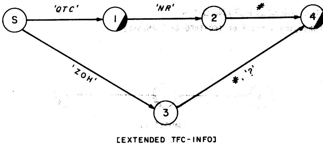
Figure 10c: Extended TFC-INFO
