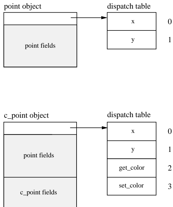
Figure 2-1: Objects and dispatch tables
