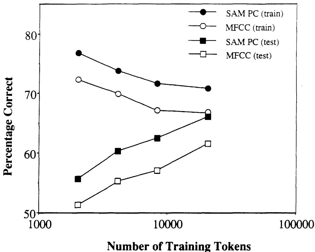
Figure 2.8: Effect of increasing training data on testing accuracies
