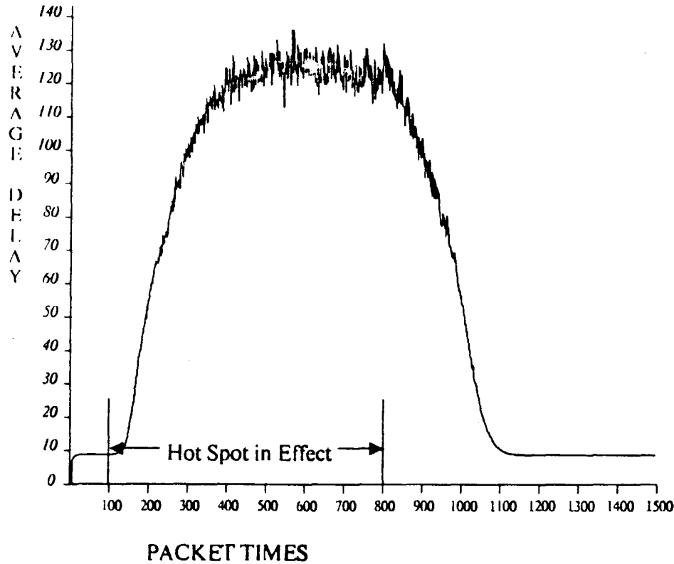
Figure 5.4: Delay in an Uncontrolled System with a 16% Hot Spot
