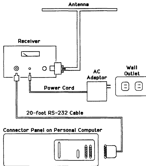
Figure I-1: Installation Diagram
