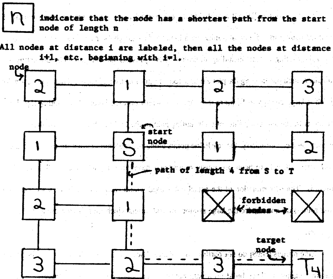
Figure 2.2: Lee's Algorithm.
