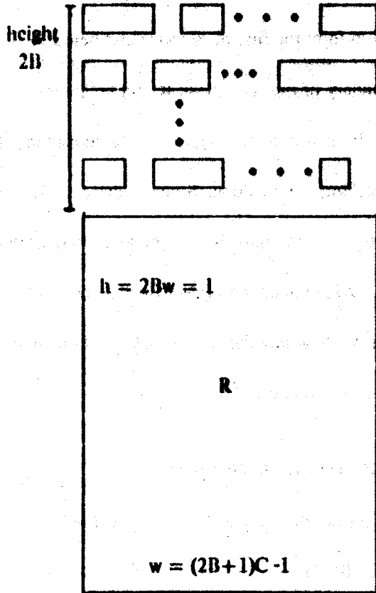
Figure 4.1: A placement given a bin packing.
