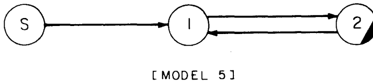
Figure 6b: A special case of Model 5
