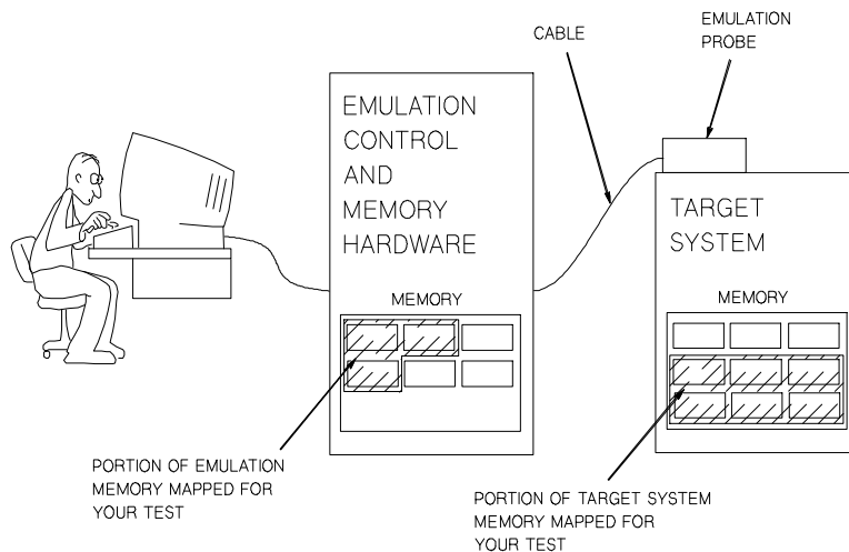
Figure 2-2. In-Circuit Emulation
