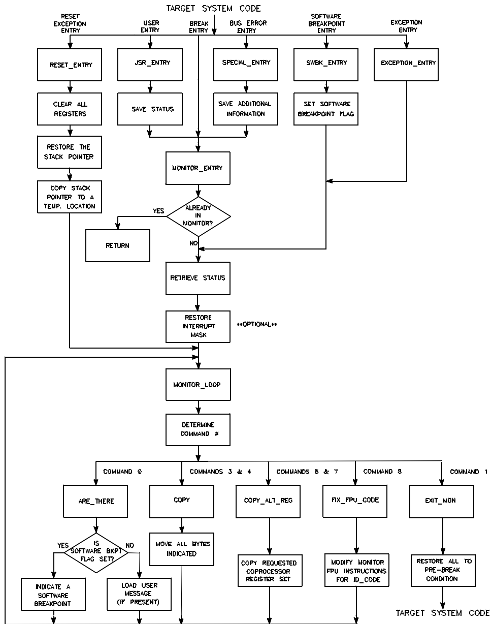
Figure 3-2. Emulation Monitor, Typical Block Diagram
