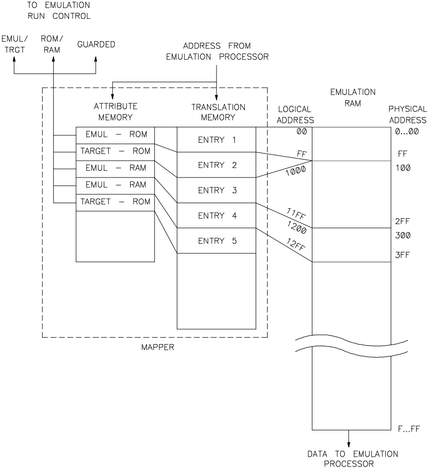
Figure 5-2. Emulation Memory Architecture
