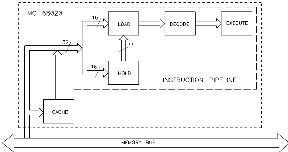
Figure 11-1. Pipeline Diagram Of The 68020
