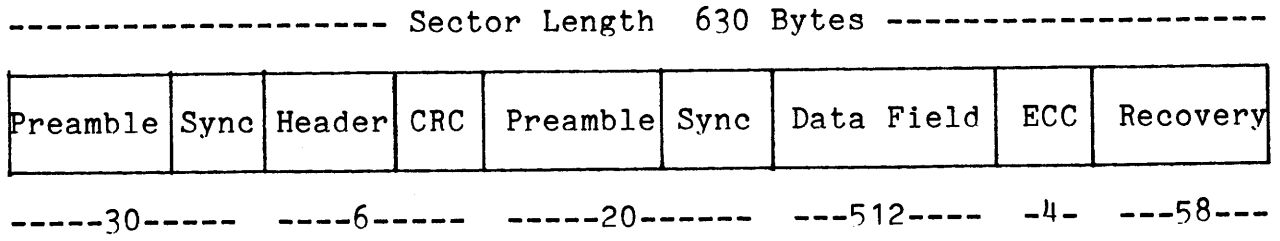
Figure 2-6 Sector Format
