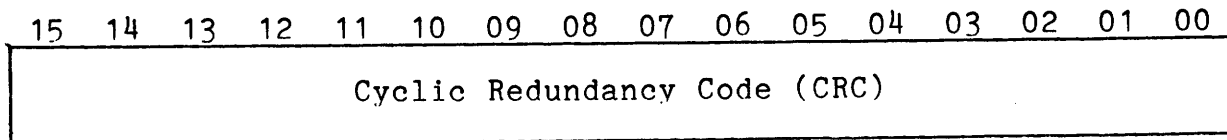
Figure 2-7 Header Format
