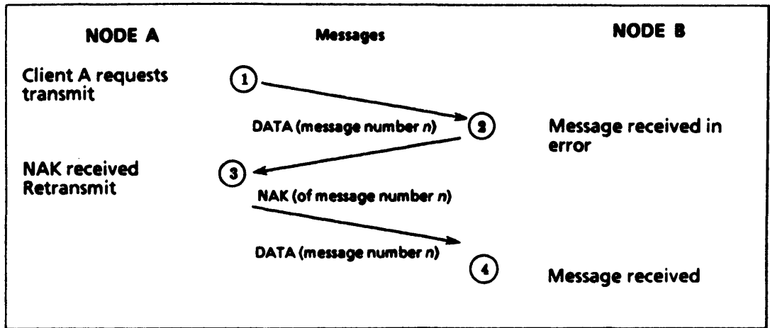
Figure 2-5: DDCMP Message Exchange, Showing Error Recovery
