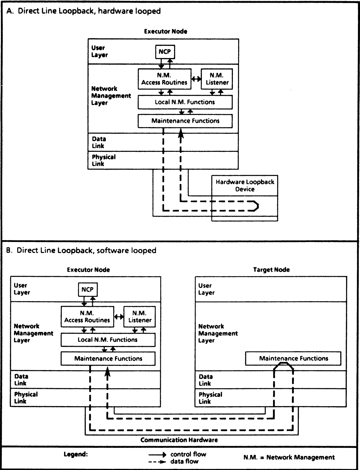
Figure 7-3: Line Loopback Tests
