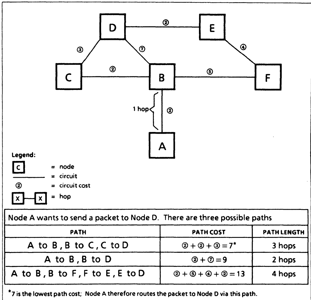
Figure 3-1: Routing Terms
