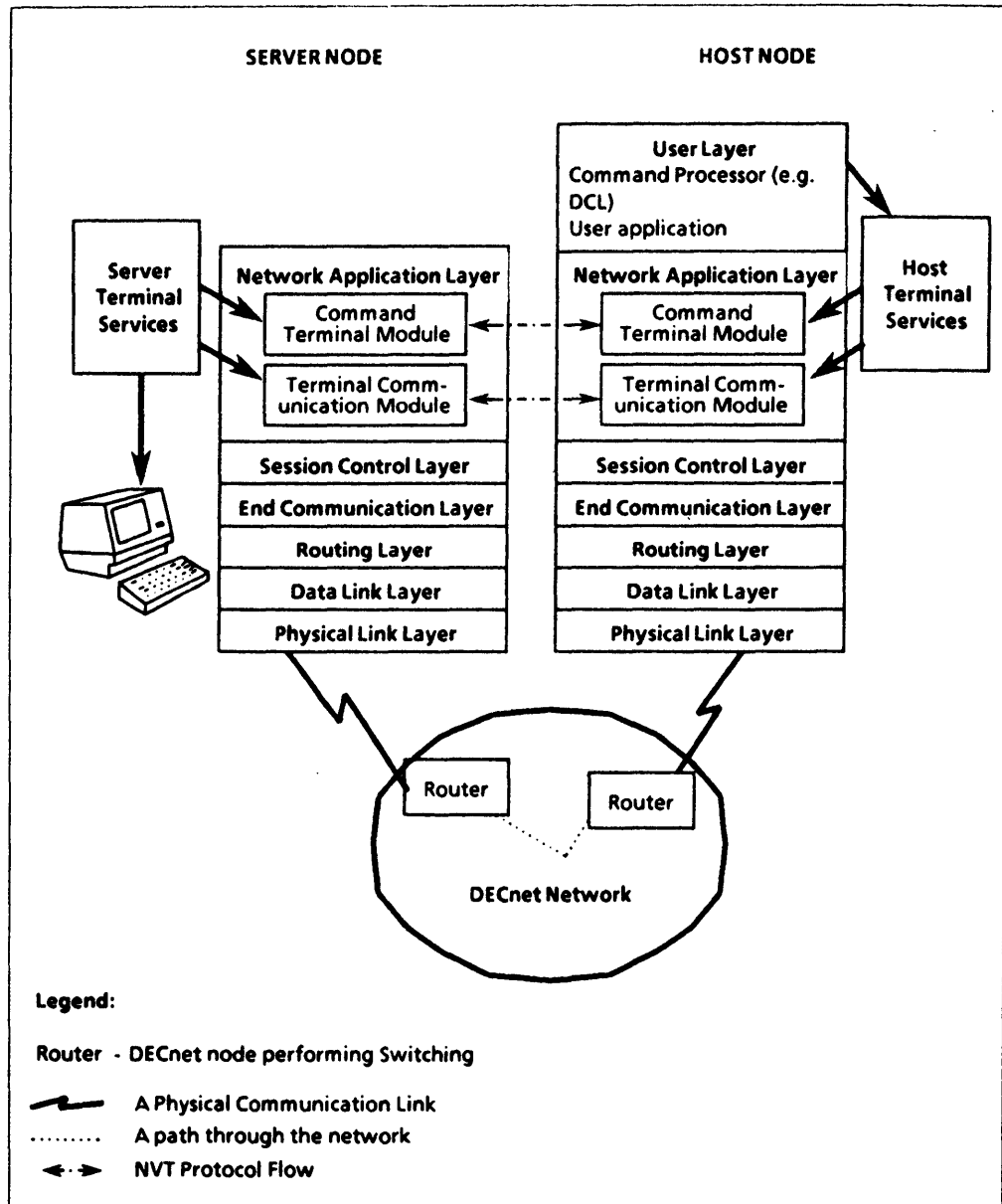
Figure 6-3: Network Virtual Terminal Service
