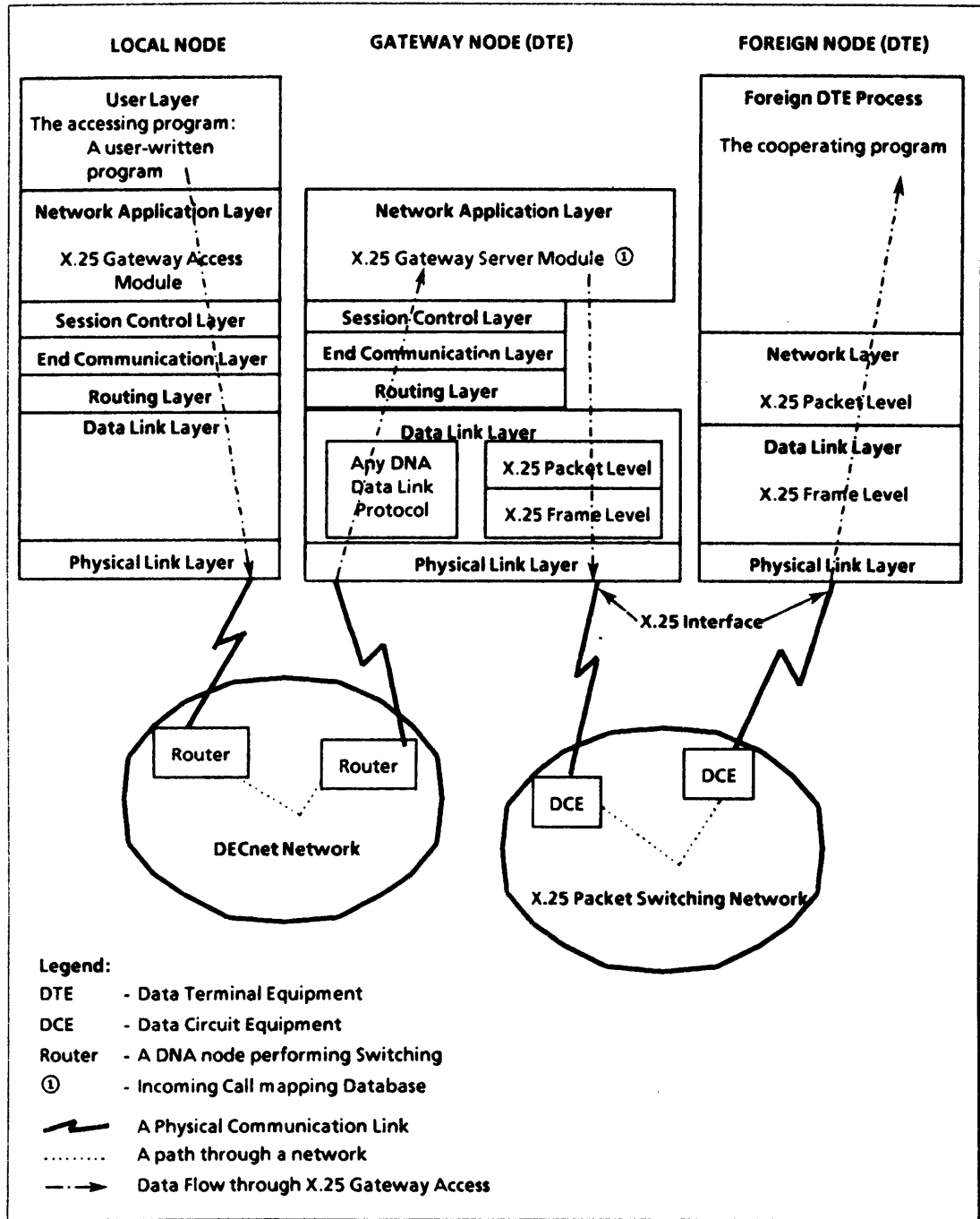
Figure 6-6: X.25 Gateway Access Operation
