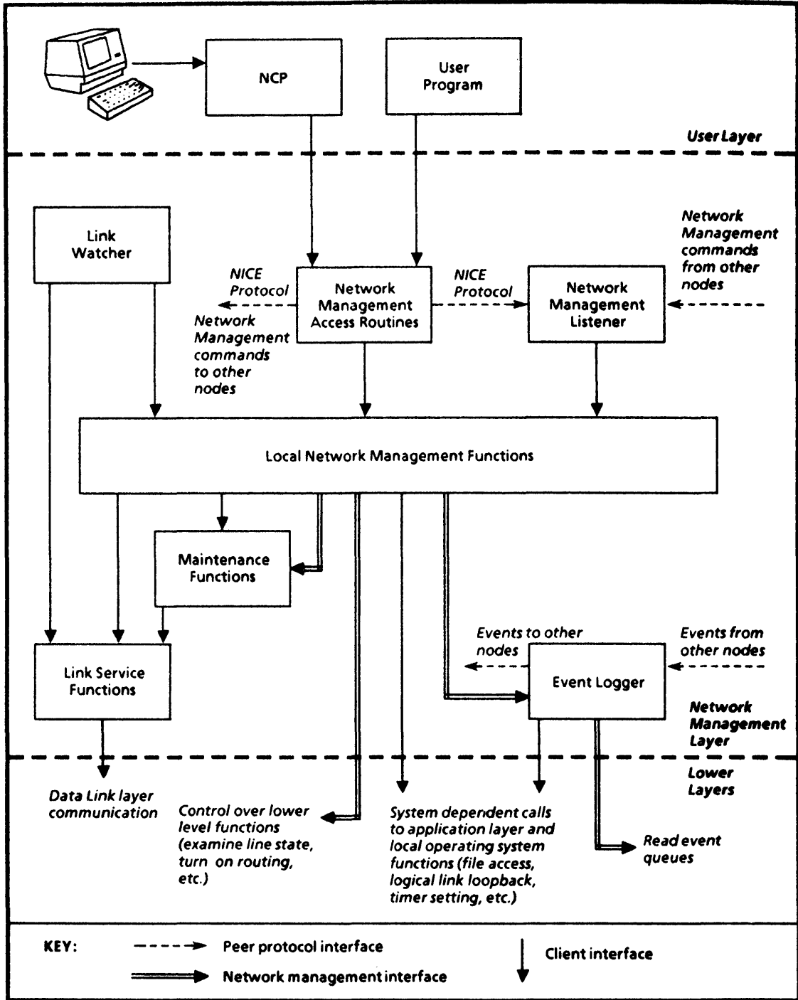
Figure 7-1: Relationship among Network Management Components at a Single Node
