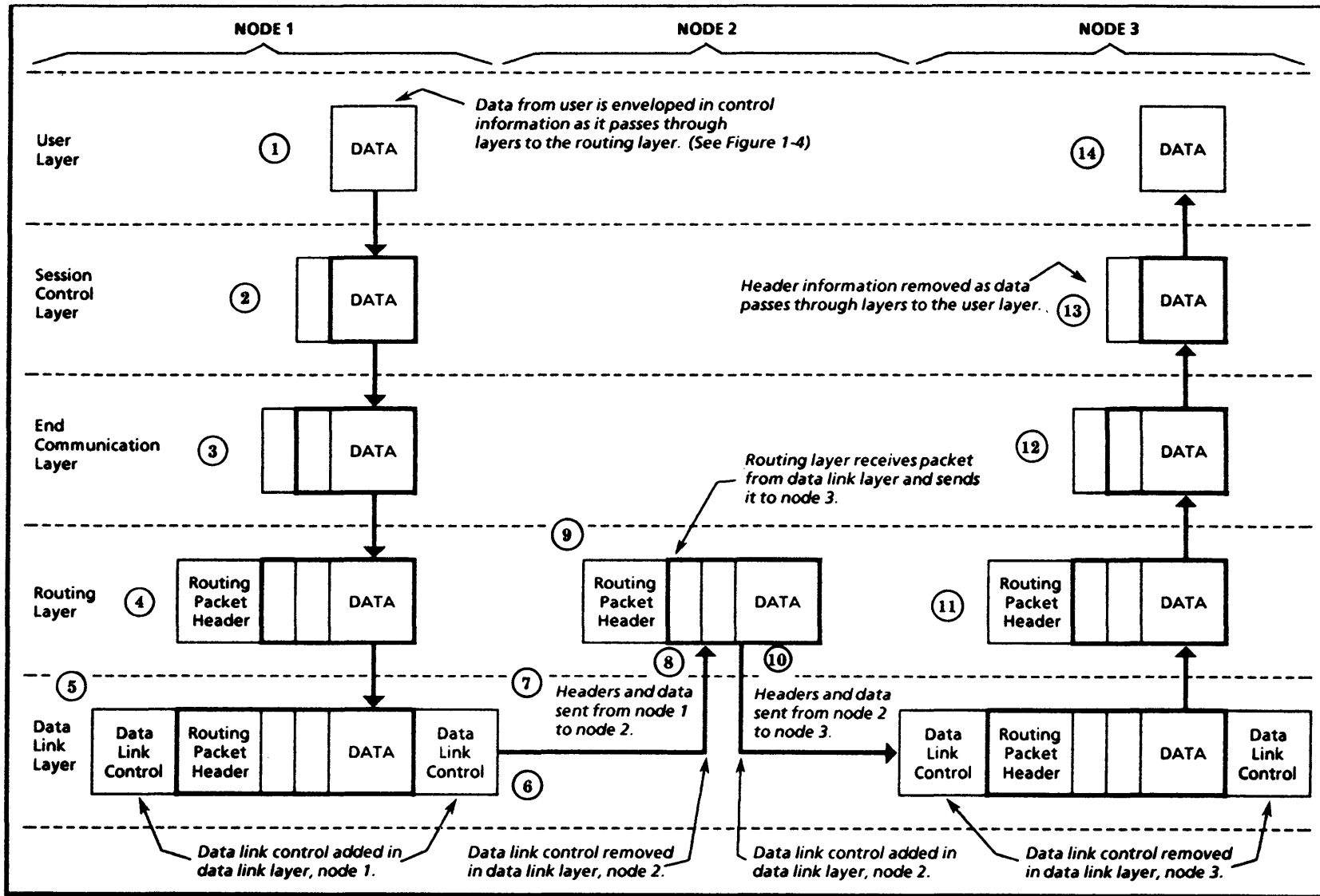
Figure 1-6: Data Flow
