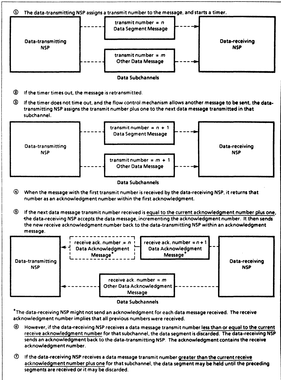
Figure 4-3: Acknowledgment Operation
