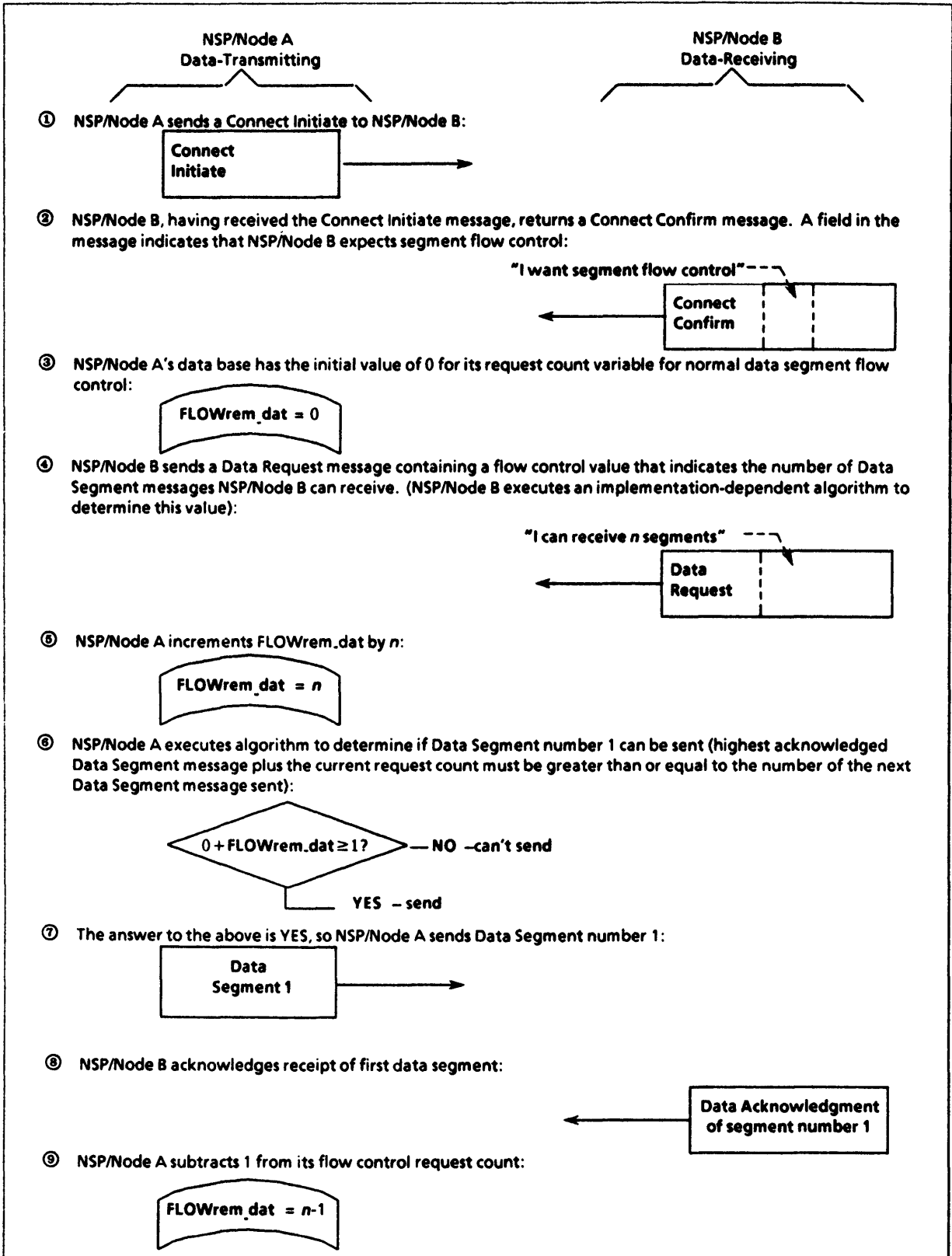
Figure 4-4: Segment Flow Control Shown in One Direction on a Logical Link
