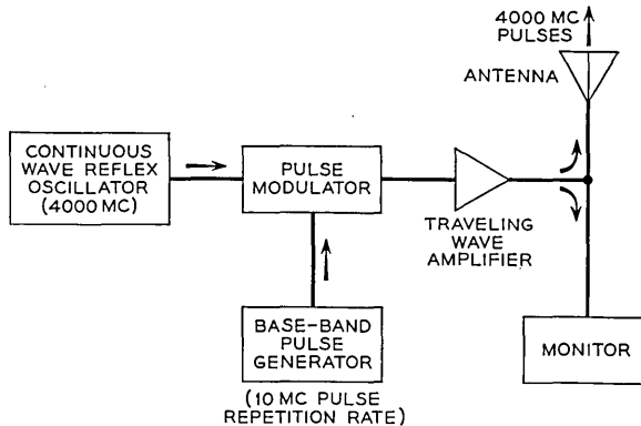
Fig. 1—Transmitting equipment.
