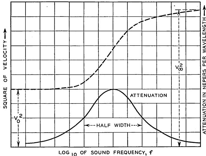
Fig. 1A—Velocity and attenuation for a medium with one relaxation frequency.
