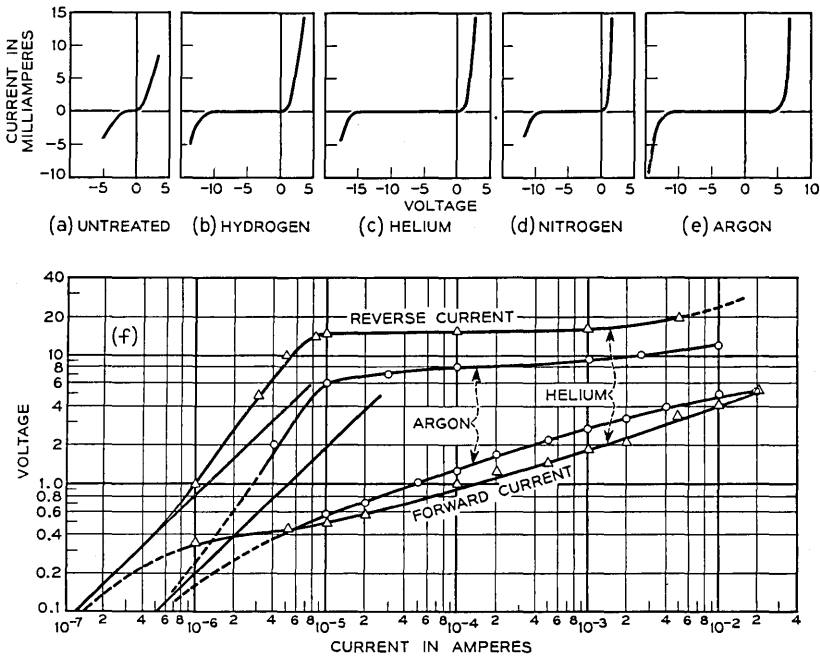
Fig. 4—Characteristics showing effect of various gases all with a bombarding potential of 30 kv.
