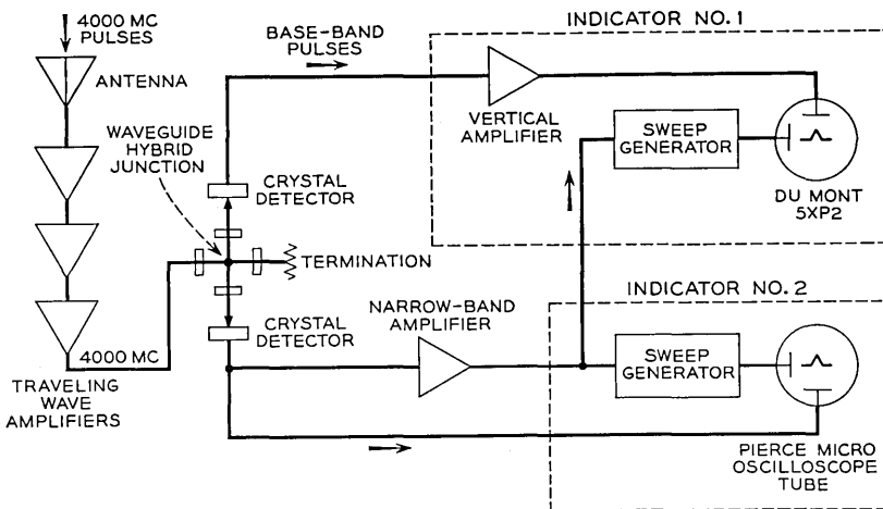
Fig. 2—Receiving equipment.
