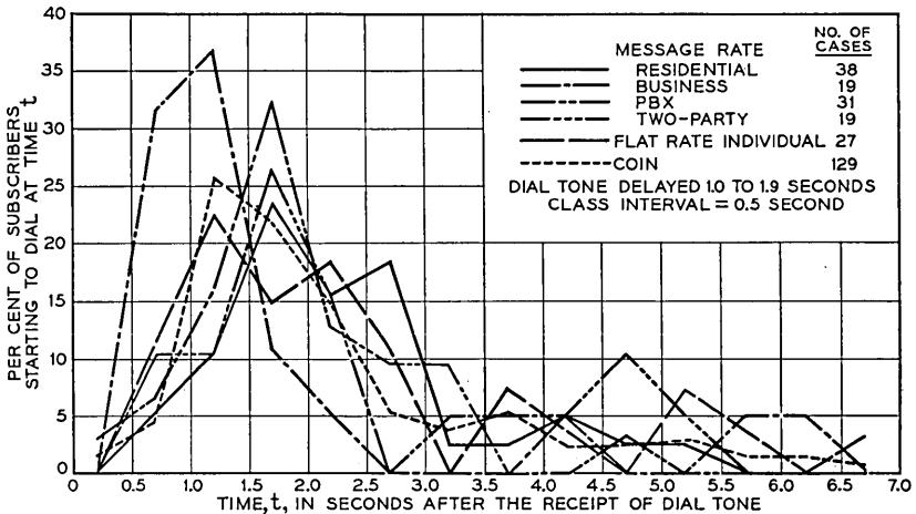
Fig. 22—Distributions of the start-to-dial times of subscribers who dial after the receipt of dial tone.
