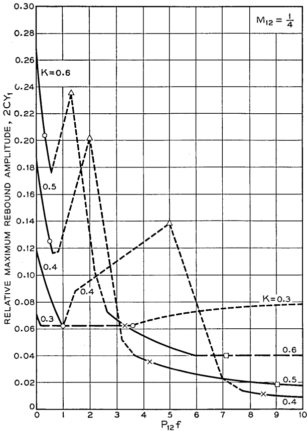
Fig. 7—Relative maximum rebound amplitude for M_{12} = 1/4 .
