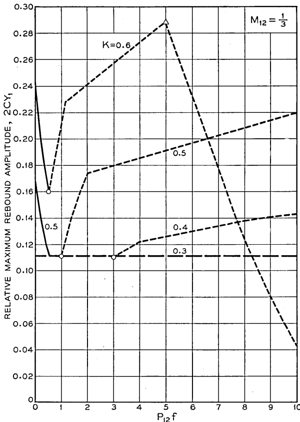
Fig. 6—Relative maximum rebound amplitude for M_{12} = 1/3 .
