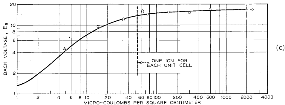
Fig. 7—Effect of time and bombarding charge on back voltage.
