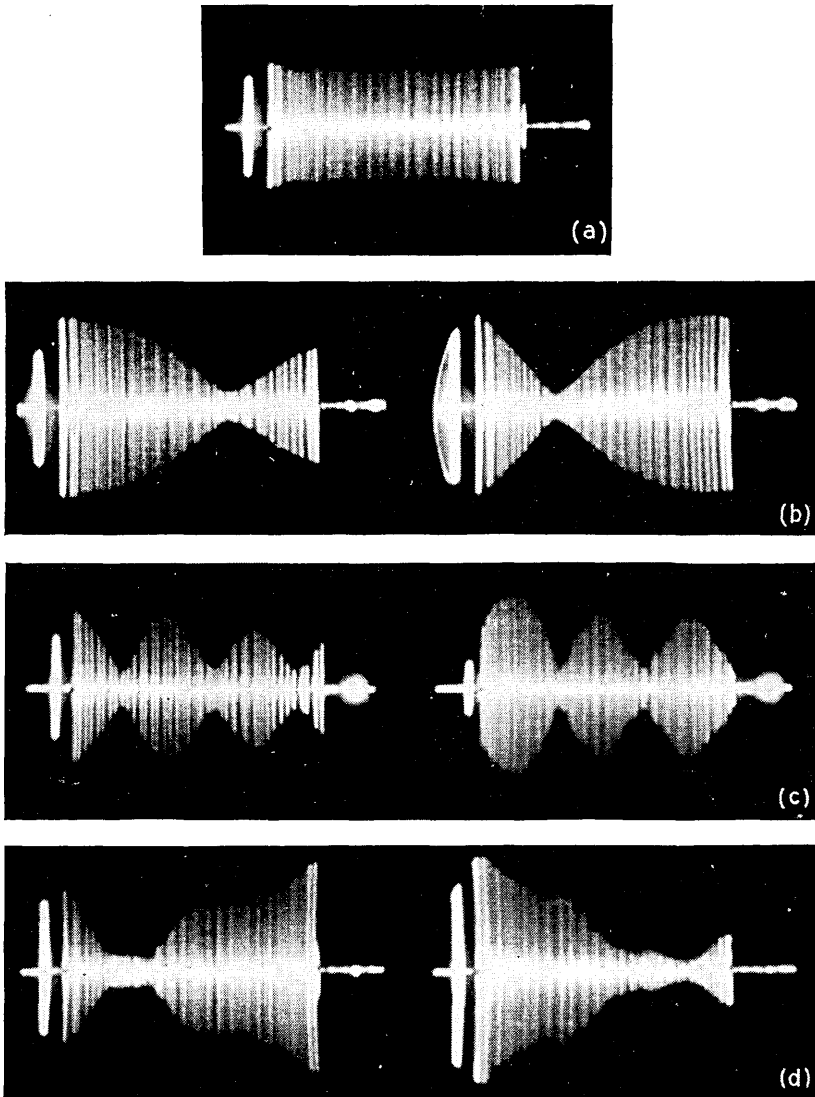
Fig. 7—Representative frequency-sweep patterns observed on the Murray Hill-Crawford Hill path. (Summer 1949.) (a) Normal day. (b) Two components with a path difference of two feet. (c) Two main components with a path difference of about six feet plus a small third component. (d) Multiple component pattern.
