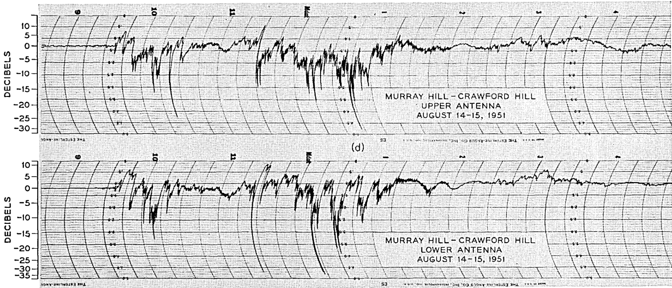
[Fig 11.—Typical recordings of 4195-mc transmission during severe fading conditions. The zero decibel line represents the normal daytime (free space) level. (a) Substandard conditions on the Southard Hill-Crawford Hill path. Night of Oct. 21-22, 1950. (b) Multiple path transmission on the Murray Hill-Crawford Hill path. Night of Aug. 26-27, 1950. (c) Multiple path transmission on a night when abnormal water reflections were present on the Murray Hill-Crawford Hill path. Night of Sept. 8-9, 1950. (d) Simultaneous recording of the outputs of two similar antennas; vertical spacing of 30 feet. Night of Aug. 14-15, 1951.
