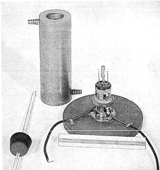
Fig. 2—Cell and 80-kc crystal for shear viscosity and elasticity measurements of liquids.
