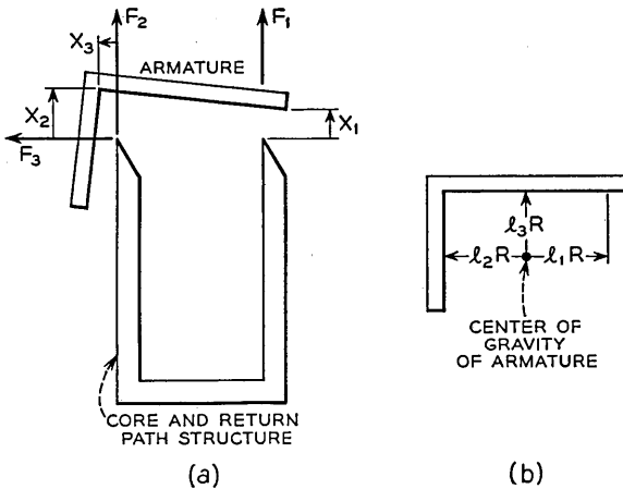
Fig. 3—Armature system—three degrees of freedom.
