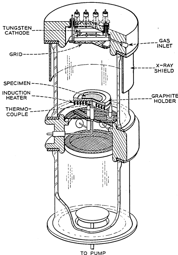
Fig. 1—Bombardment apparatus.
